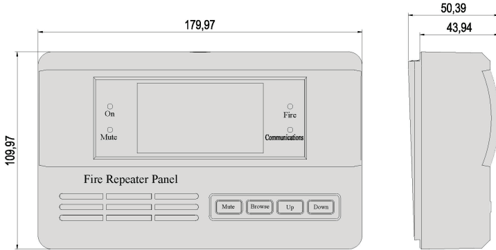
Figure 1: LCD Repeater Panel Structure
